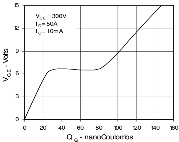
Fig. 11. Gate Charge
